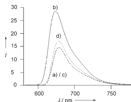
Figure 6. Fluorescence spectra ( \text{CDCl}_3/\text{CD}_3\text{CN} (1:1), 298 K; excitation at 400 nm) of a) an equimolar mixture ( 1.3 \times 10^{-4}\text{ M} ) of 1 and 4 , b) the system in (a) after the addition of 2 equiv of \text{NaClO}_4 , c) the system in (a) after the addition of 2 equiv of \text{KPF}_6 , and d) the system in (b) after the addition of 20 equiv of \text{KPF}_6 .
