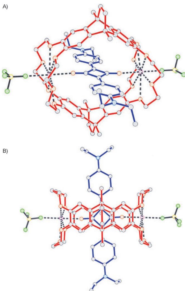
Figure 4. Ball-and-stick representations of the solid-state structure [\mathbf{4} \subset \mathbf{1} \supset \text{Na}_2][2\text{BF}_4] . Atom labels: C, gray; O, orange; N, blue; Na, purple; B, yellow; F, green.
