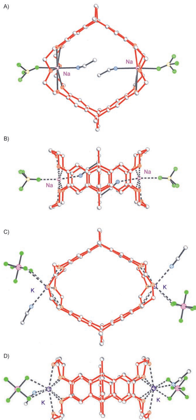
Figure 7. Ball-and-stick representations of the solid-state structures of [(1DNa_2) \cdot 2 MeCN][2 BF_4] : a) side view; b) top view, and [(1DK_2) \cdot 2 MeCN][2 PF_6] : c) side view; d) top view. Atom labels: C, gray; O, orange; N, blue; Na, light purple; B, yellow; P, pink; K, purple; F, green.
